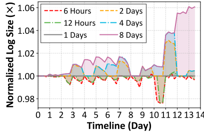
Fig. 21. Impact of update frequency on AdaLog's storage efficiency. For better comparison, behavior log sizes are normalized against the size achieved under a standard daily update schedule.
